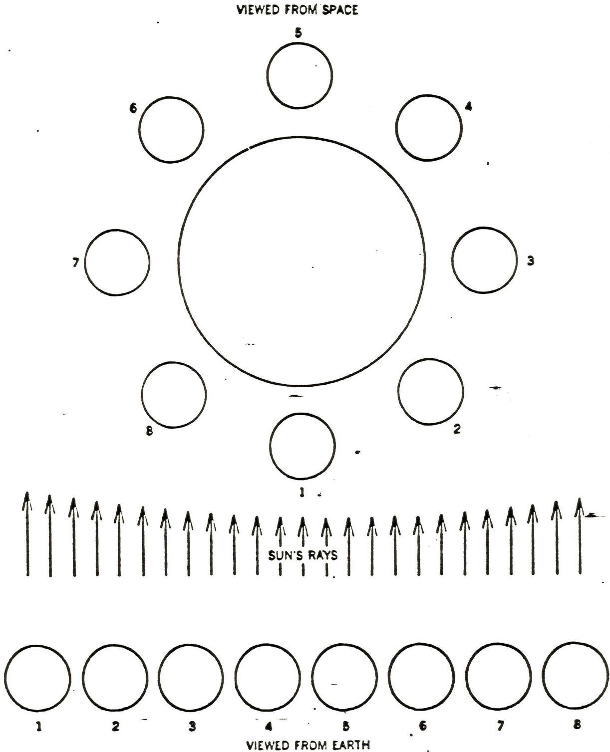
Figure 27-1 Phases of the moon
